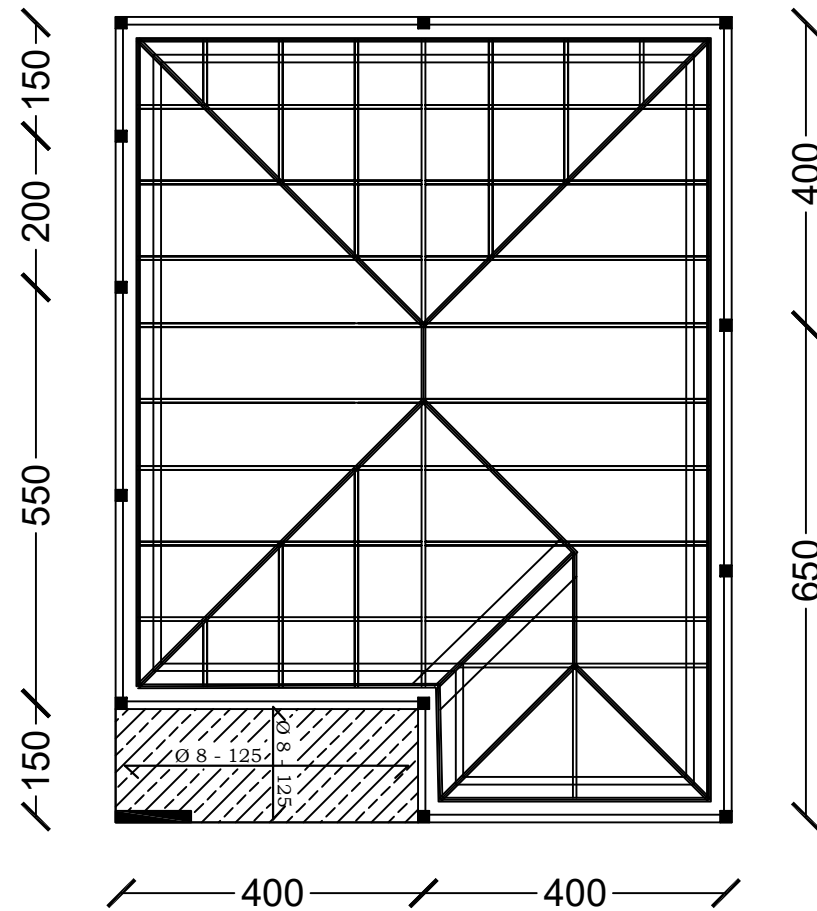
DENAH ATAP LT2 SKALA 1 : 100
